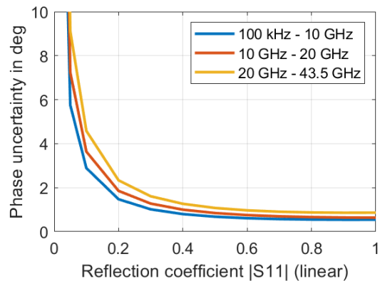
Typical uncertainty of reflection magnitude and reflection phase measurements of the R&S®ZNB43, in the frequency range from 100 kHz to 43.5 GHz; analysis conditions: S_{12} = S_{21} = 0 , cal. power -10 dBm, meas. power -10 dBm
