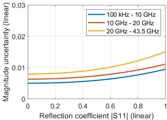
Typical uncertainty of reflection magnitude and reflection phase measurements of the R&S®ZNB43, in the frequency range from 100 kHz to 43.5 GHz; analysis conditions: S_{12} = S_{21} = 0 , cal. power -10 dBm, meas. power -10 dBm
